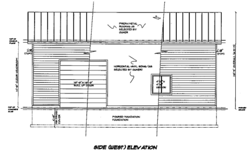
SIDE (WEST) ELEVATION
