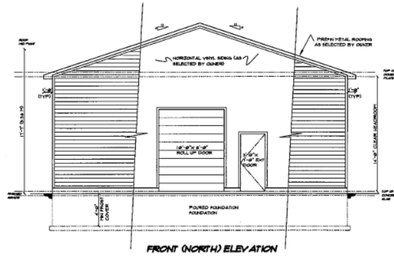
FRONT (NORTH) ELEVATION
