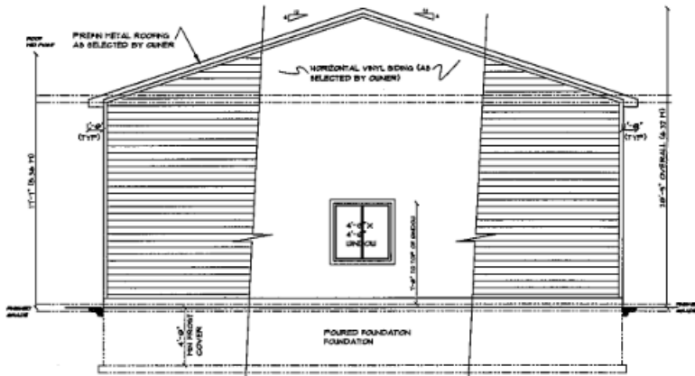
REAR (SOUTH) ELEVATION
