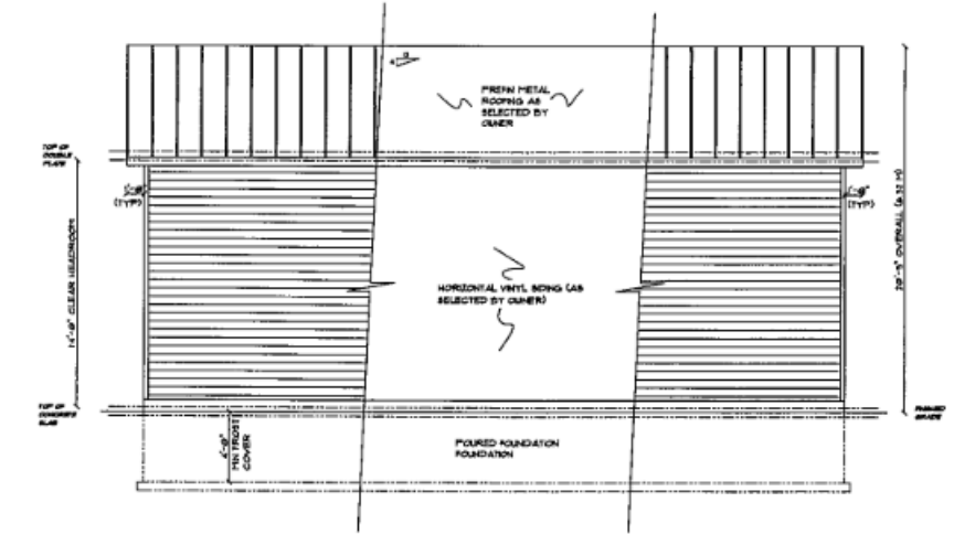
SIDE (EAST) ELEVATION
